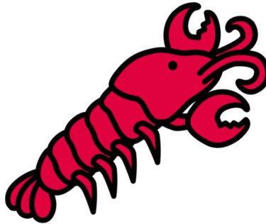
11. lobster
