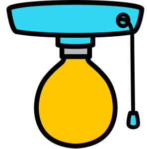
9. light bulb
