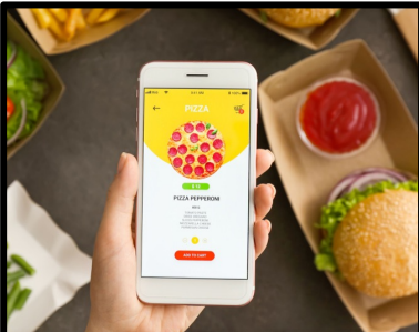
7. order food
